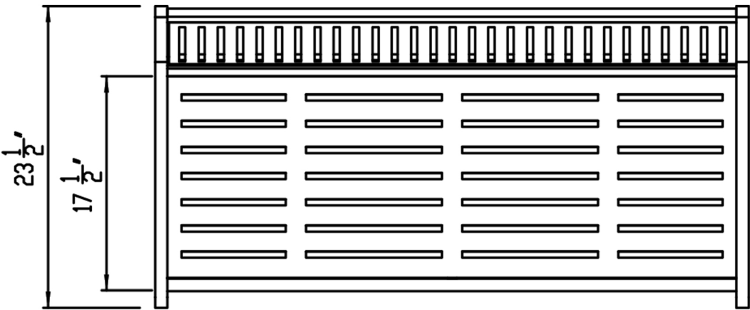
TOP VIEW
