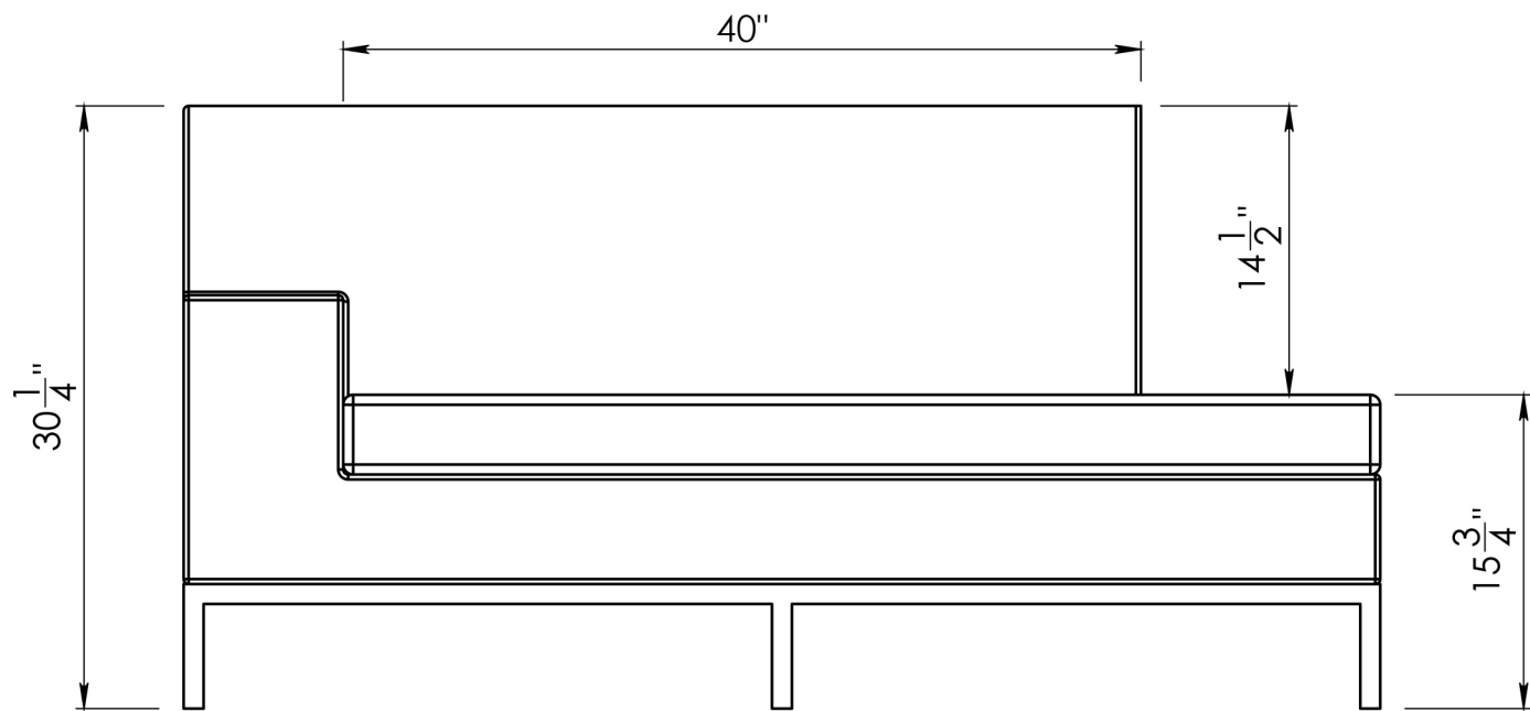
FRONT VIEW
