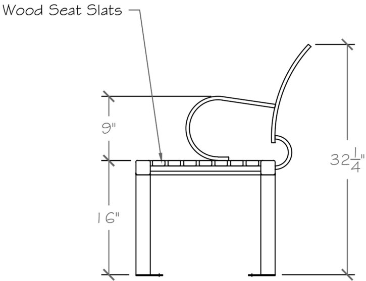
SECTION VIEW
